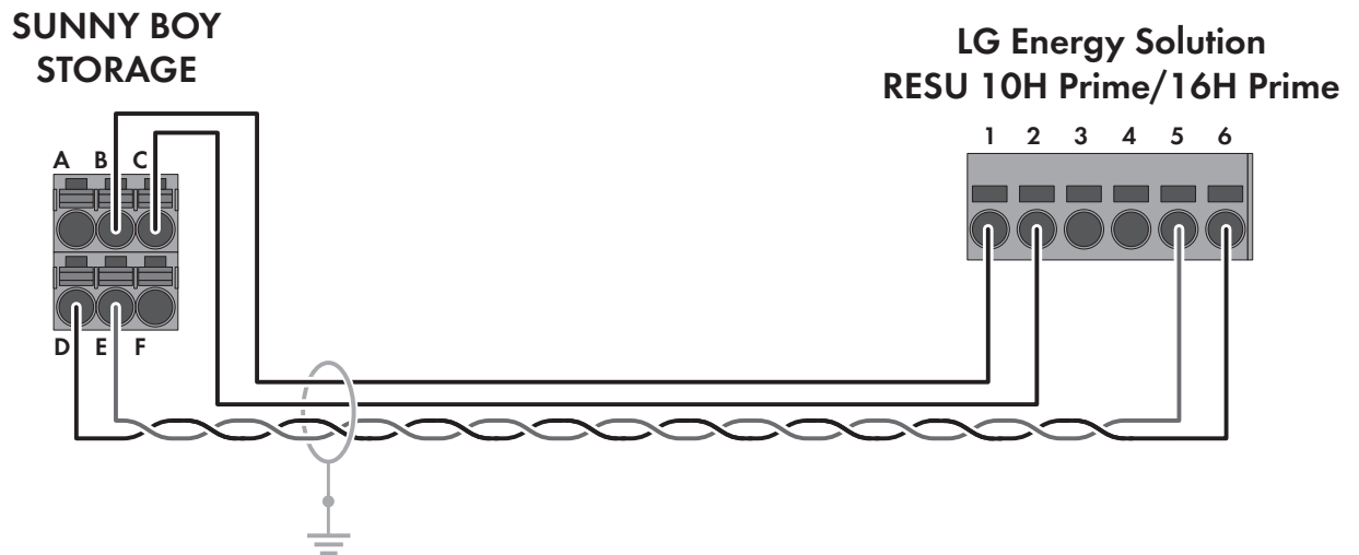
Figure 5: Cabling plan SBS3.7-10 / SBS5.0-10 / SBS6.0-10 with RESU 10H Prime / 16H Prime
